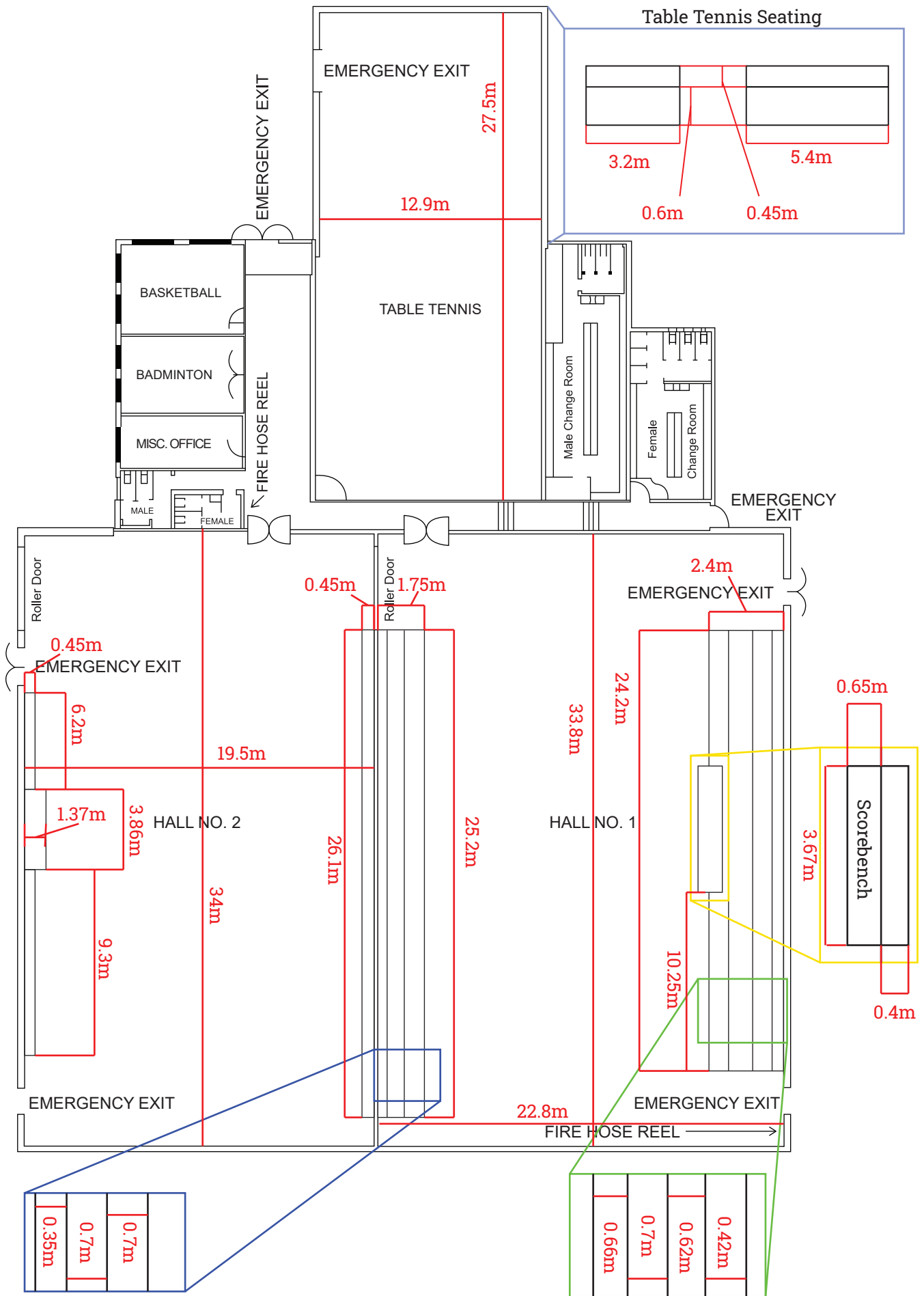
Drawing Not to Scale
